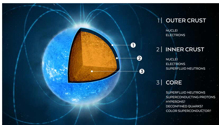
Figure 7: Cross section of a neutron star, showing the composition for each of its layers. Figure taken from [499].
