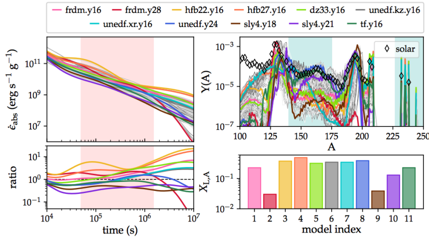
Figure 5: Impact of nuclear physics uncertainties on r -process nucleosynthesis and kilonovae [335]. As described in Table 1 of [336] and Table 2 of [335], the labels provide short-hand notation for the different mass models / fission barrier models applied (FRDM2012 [337] / FRLDM [338], HFB22 [339] / HFB14 [340], HFB27 [341] / HFB14, Duflo-Zuker [342] / FRLDM, UNEDF1 [343] / FRLDM, SLY4 [344] / FRLDM, and Thomas Fermi [345] / Thomas Fermi [346]) as well as the neutron-richness considered for each case (for example .y16 implies Y_e = 0.16 ). Absolute nuclear heating rate is shown (top left) as well as a ratio comparison to a power law assumption (bottom left) for all cases considered. The variances in the predicted nucleosynthetic abundances are shown as a function of mass number (top right) with a comparison of their total mass fractions (bottom right) of lanthanides + actinides (which are important contributors to the opacity).
